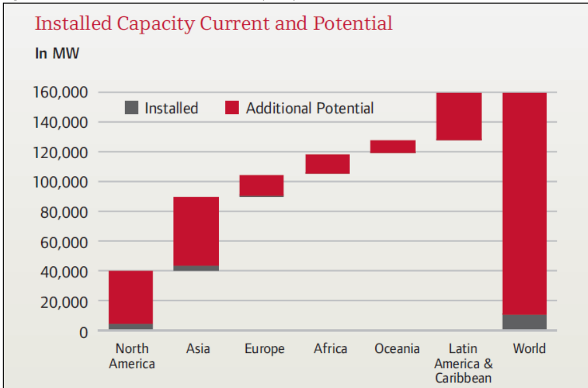
Figure 6.0 - Global Geothermal Installed Capacity & Potential (does not include Canada)
